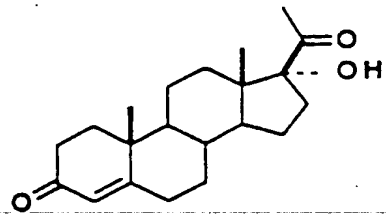
17alpha-Hydroxyprogesterone
